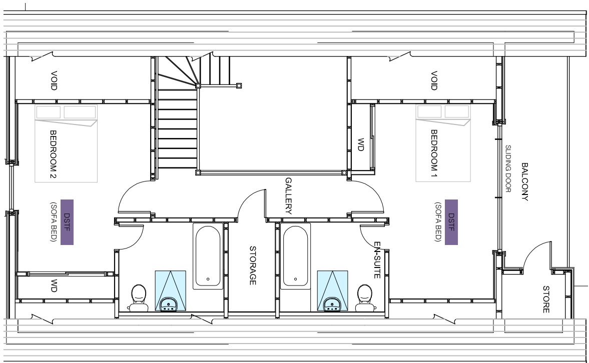
FIRST FLOOR
